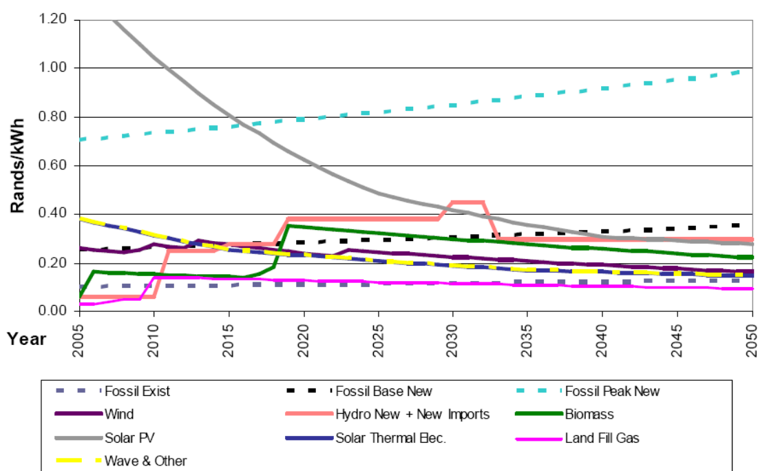
Figure 33: Progressive Renewable Scenario: Illustration of the possible changes in cost per unit energy over time. (Source: Banks and Schaffler, 2006).
