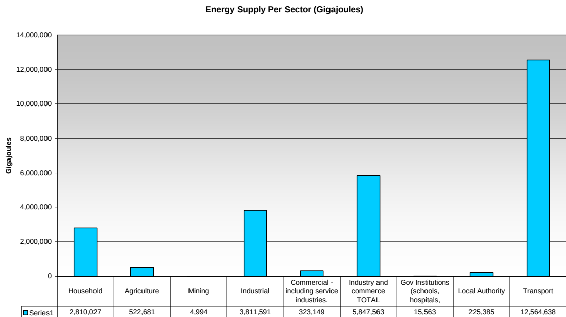
Figure 12: Energy consumption by sector.
