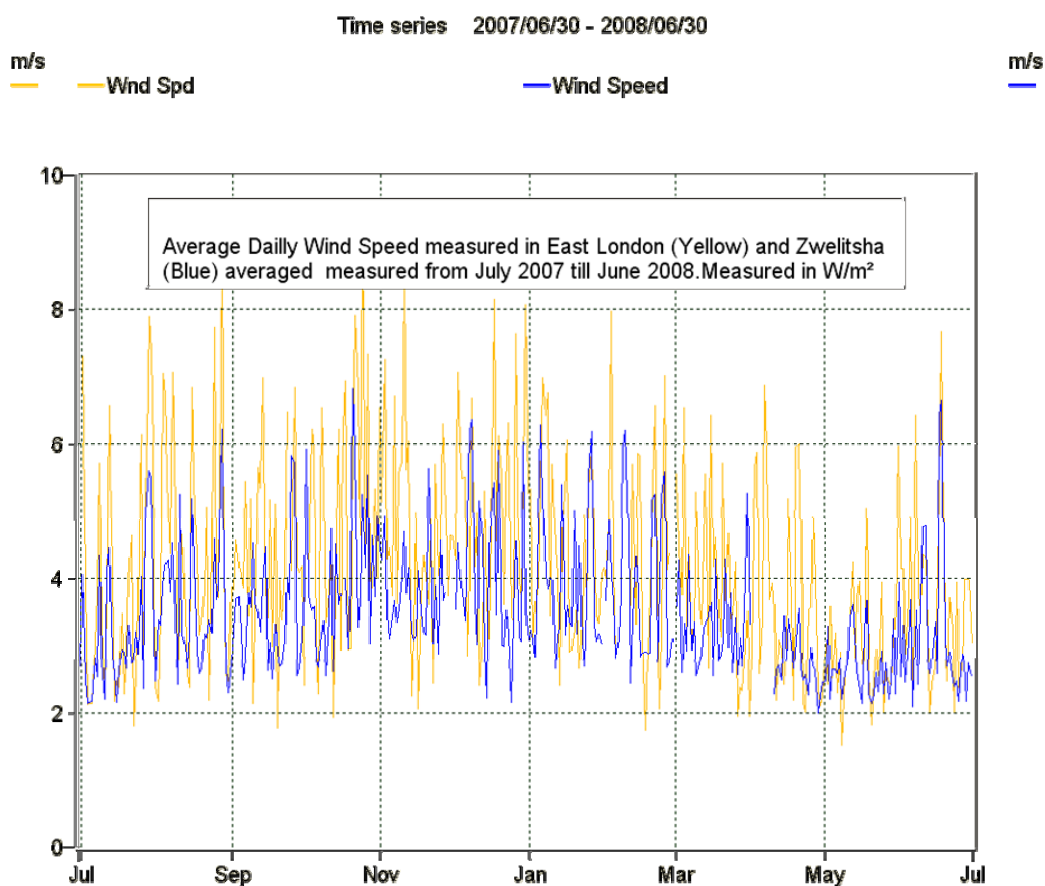
Figure 35: Average daily wind speeds in BCM taken at 10m above ground level (source: BCM Pollution Control, L. Mardon).
