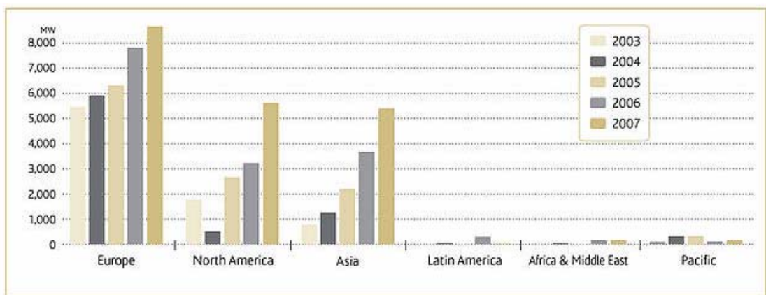
Figure 32: Annual increases in installed capacity for wind generation (2003 to 2007). Source: Global Wind Energy Council, 2008.
