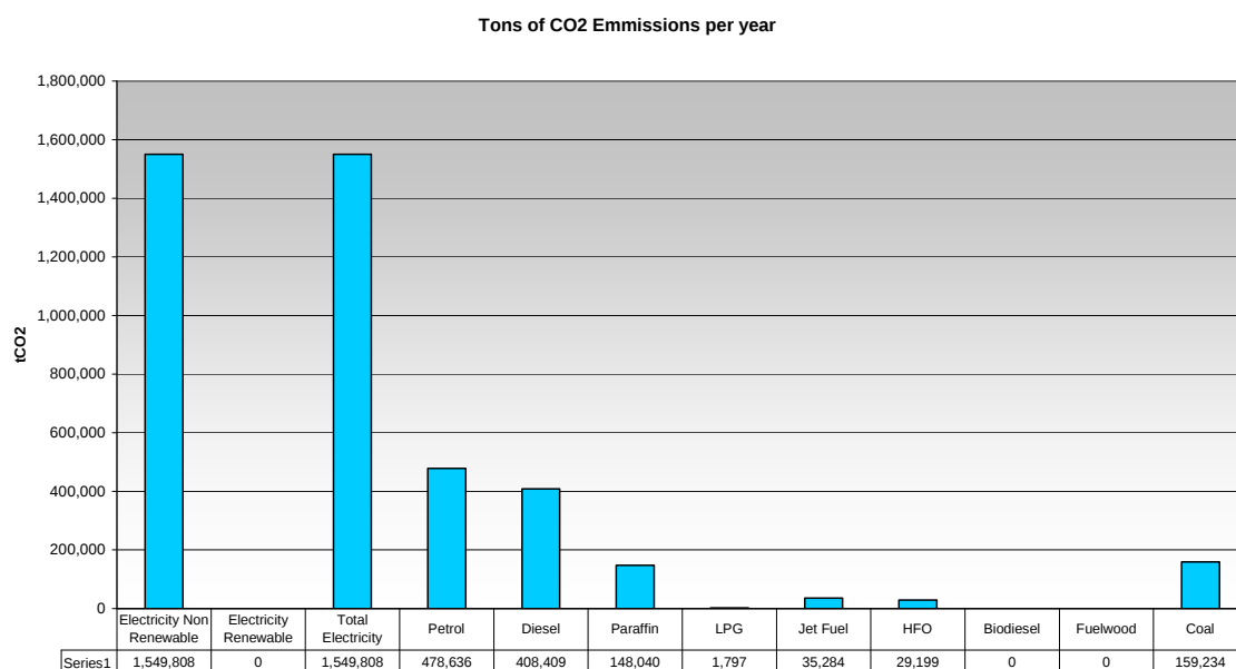
Figure 8: Global CO 2 emissions resulting from consumption of different energy types within BCM in 2007 (expressed on tons of CO 2 ).
