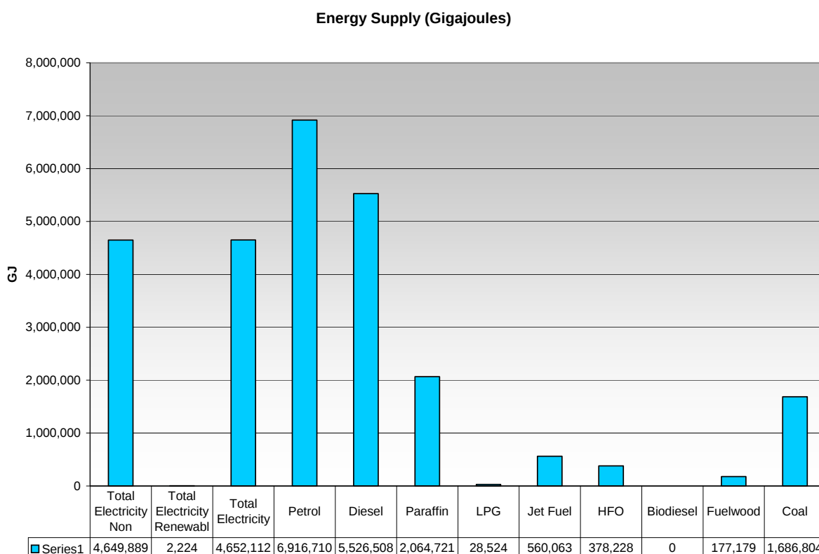
Figure 7: Integrated energy supply to BCM in 2007, expressed in Gigajoules.
