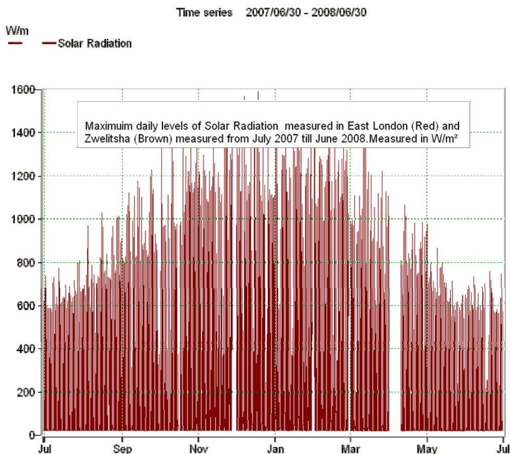
Figure 37: Solar radiation measured in BCM, measured in Watts per square metre (source: BCM Pollution Control, L. Mardon).
