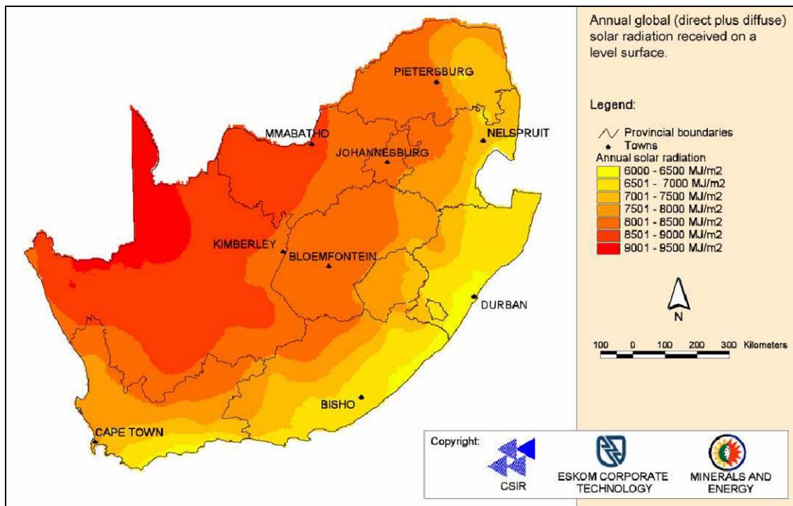
Figure 36: Incoming Solar Radiation for South Africa (DME 2003).
