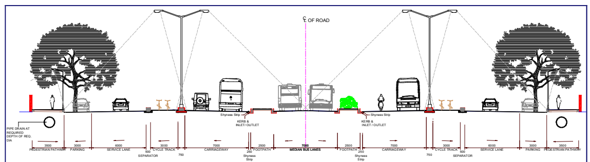
Fig. 13.104 For wide roadways with service lanes, the cycleway can be located between the service lanes and the mixed traffic lanes.
