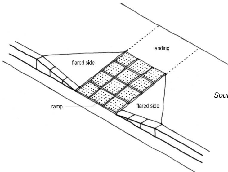
Figure 12: Kerb ramps
