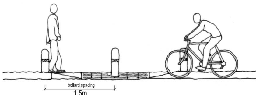
Figure 20: Bollard spacing
