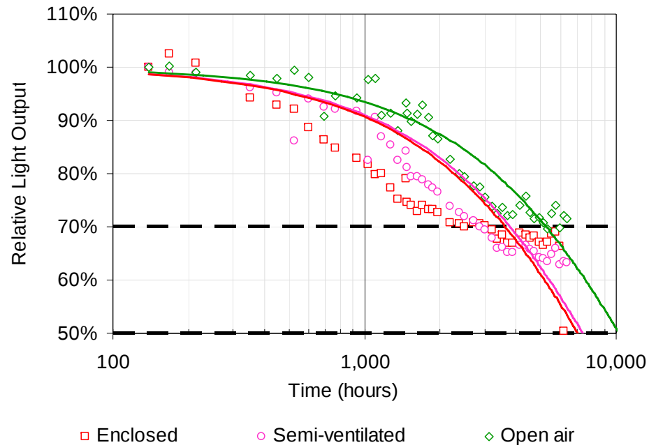
Fixture B - 26W LED Downlight
