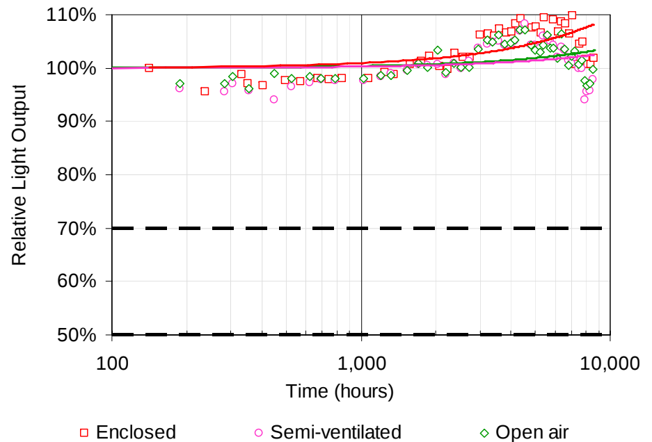
Fixture C - 12W LED Downlight
